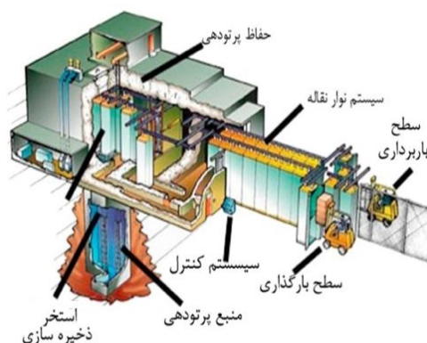
Figure 3- Gamma irradiation set up for food processing
